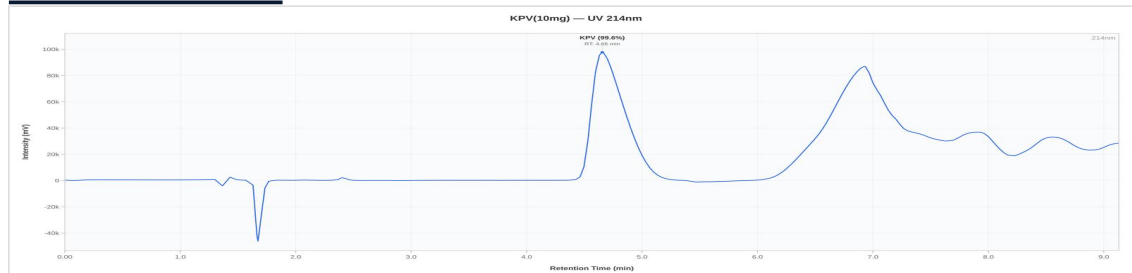
KPV 10mg - KPV260527-01: UV Chromatogram
