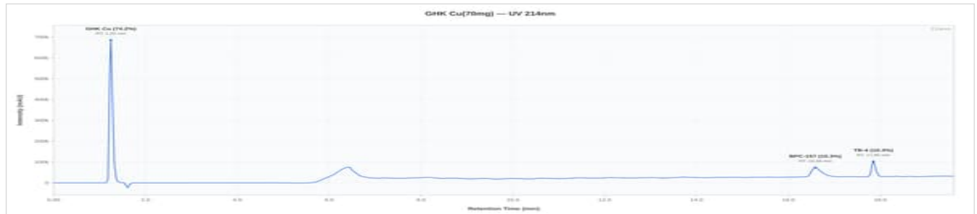
GLOW 70mg - GLO260713-01: UV Chromatogram
