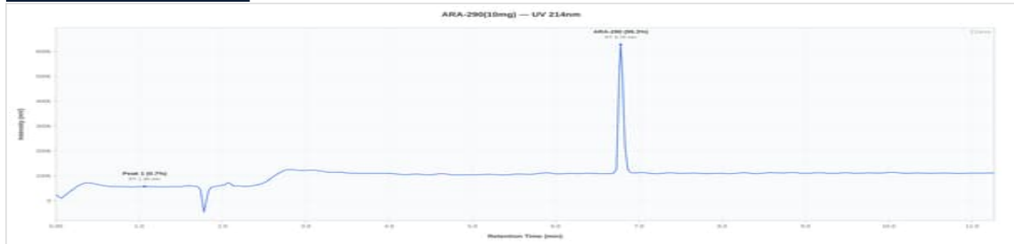
ARA-290 10mg - ARA260520-01: UV Chromatogram
