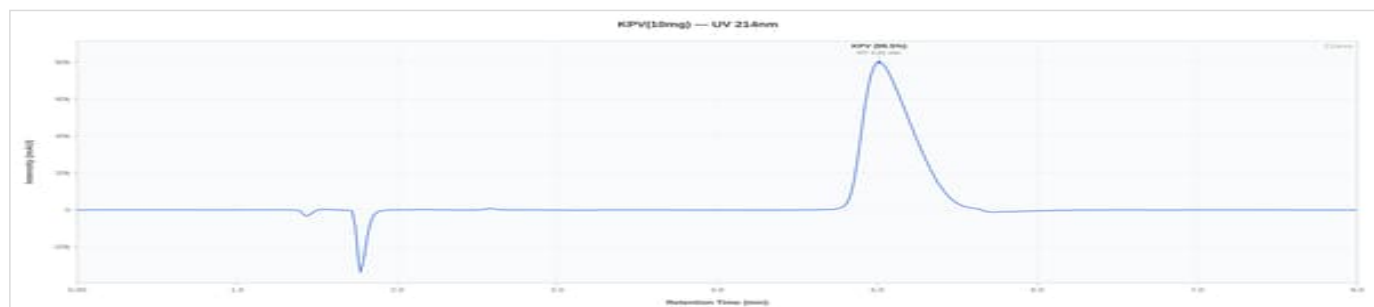
KPV 10mg - KPV260728-01: UV Chromatogram
