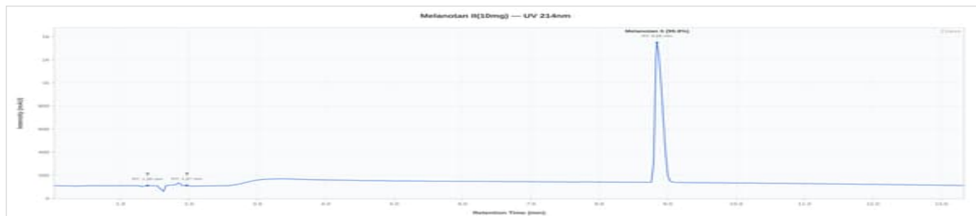
Melanotan II 10mg - MEL260713-01: UV Chromatogram
